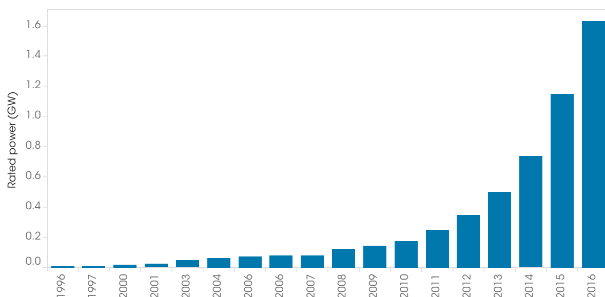
Figure 5.5 Global stationary battery storage capacity, 1996-2016
