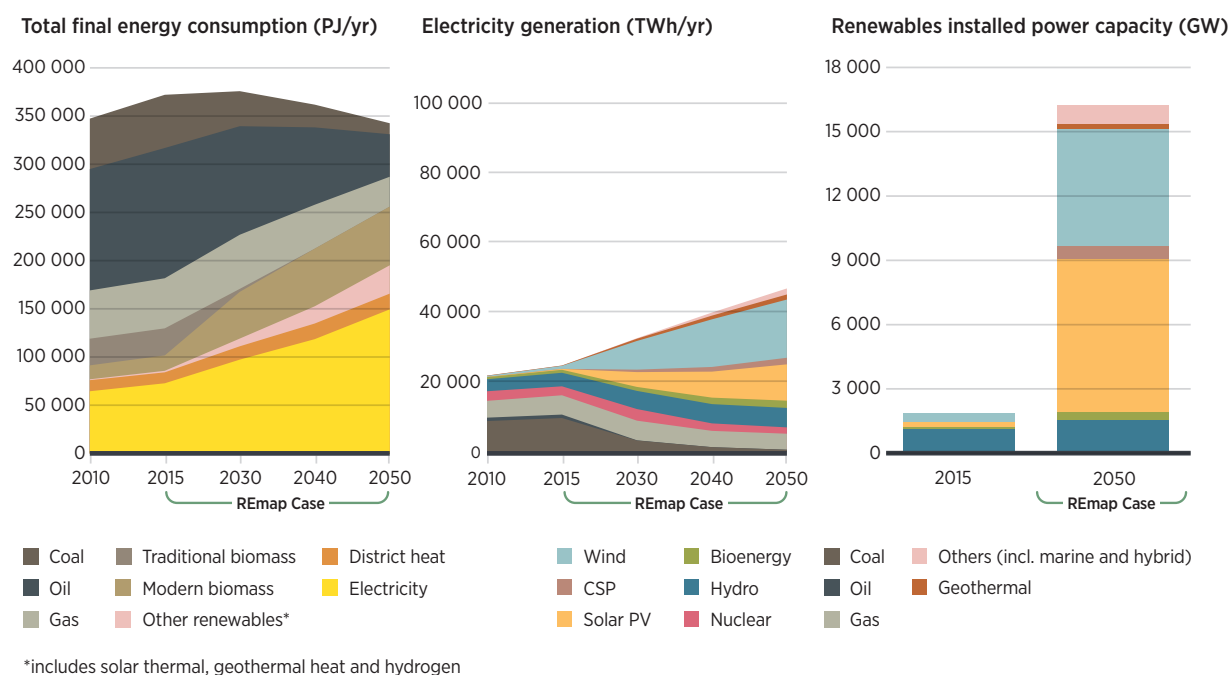
Figure 1.2 Energy consumption, electricity generation and renewable power capacity in IRENA's roadmap to 2050
