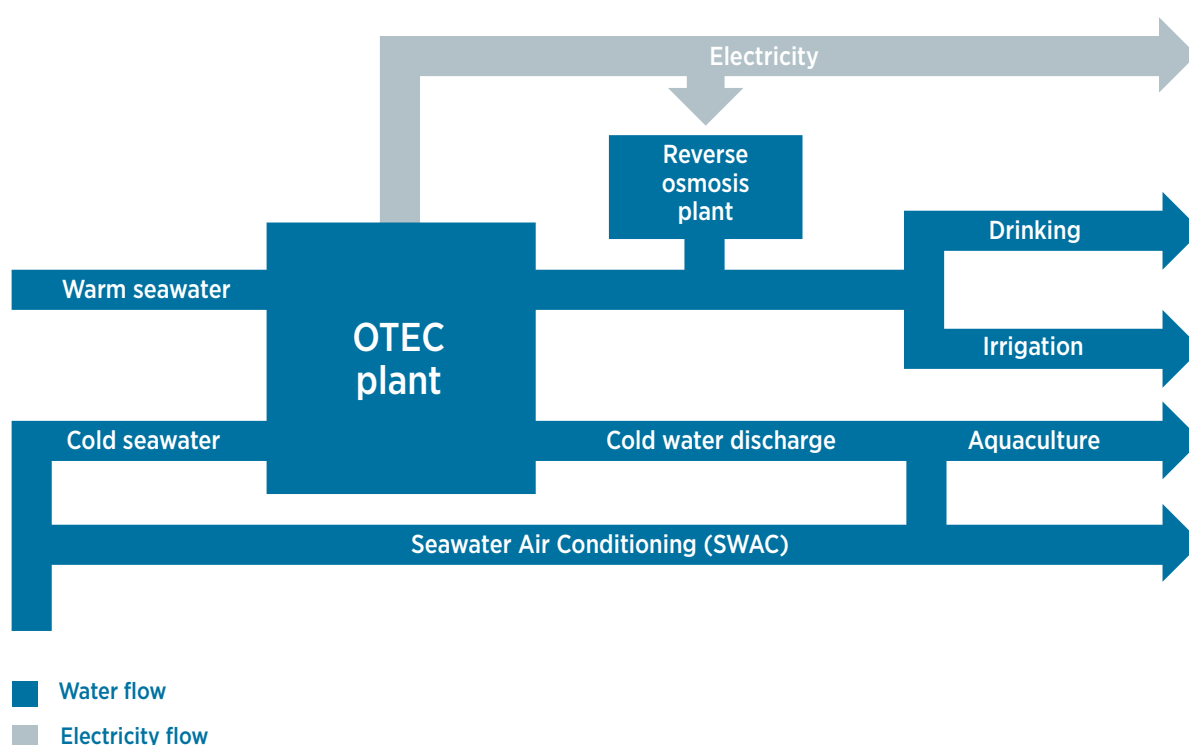
Figure 5.1 Multifunctionality of an OTEC Plant
