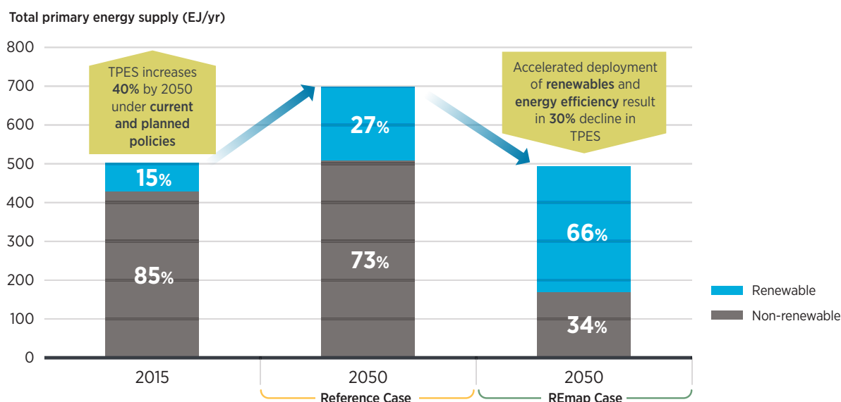
Figure 1.1 Global energy supply (TPES) and the share of renewables and non-renewables: two scenarios
