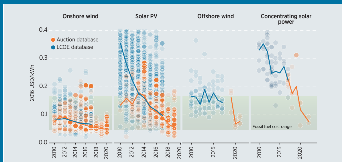
Figure 1.3 Weighted average and project-specific global LCOE from utility-scale renewable power generation technologies, 2010-2017
