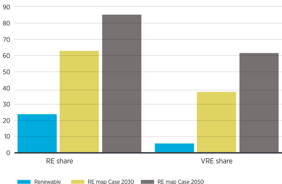
Figure 4.1 Forecasted shares of total renewable energy and variable renewable energy in total electricity generation: Two scenarios
