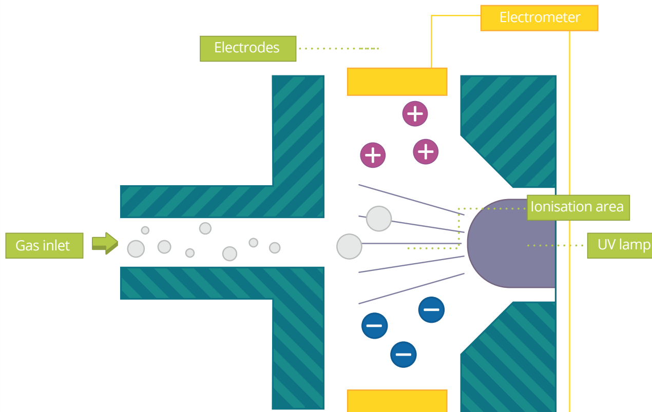
Figure 16: Schematic showing the operation of photoionisation detectors
