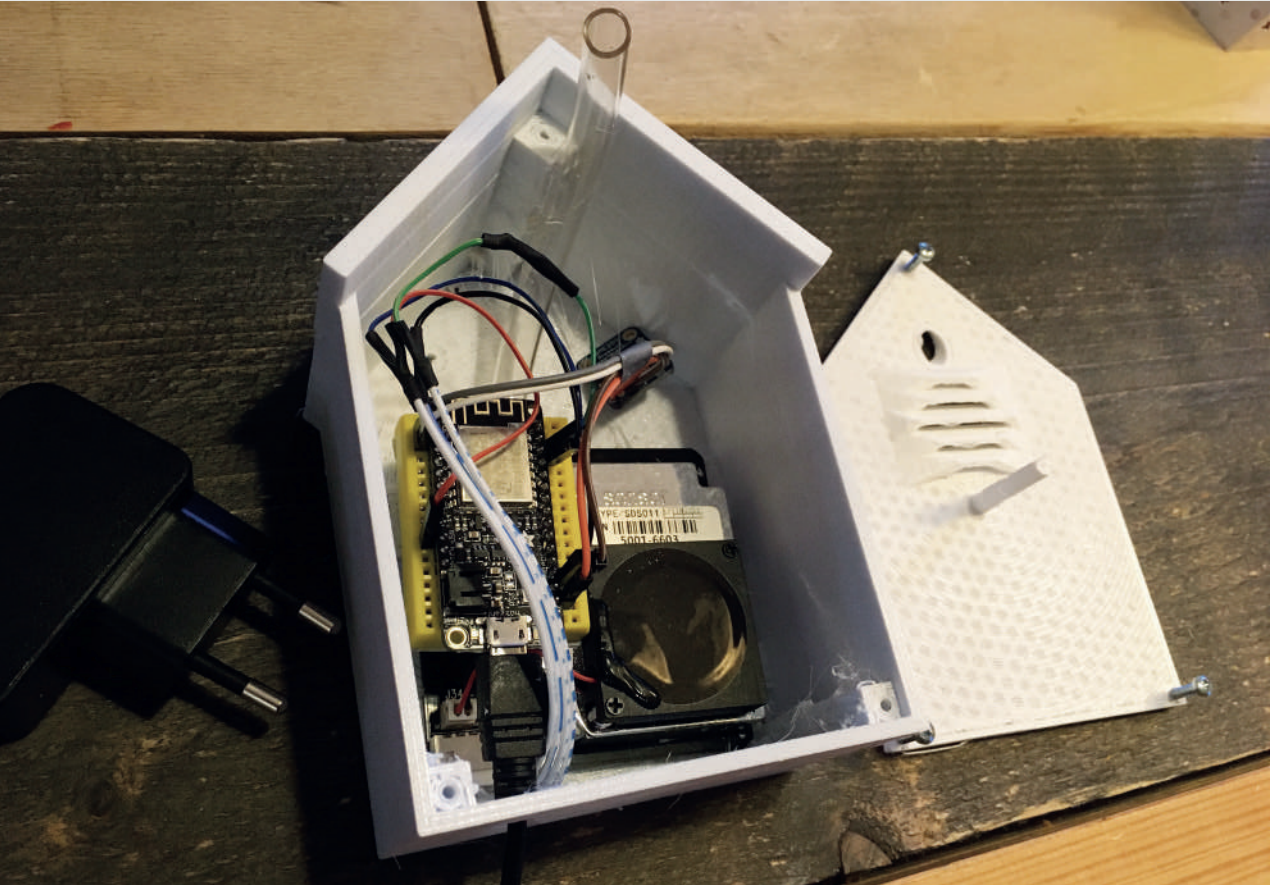
Figure 4: Example of home-made weatherproof housing for a sensor device
