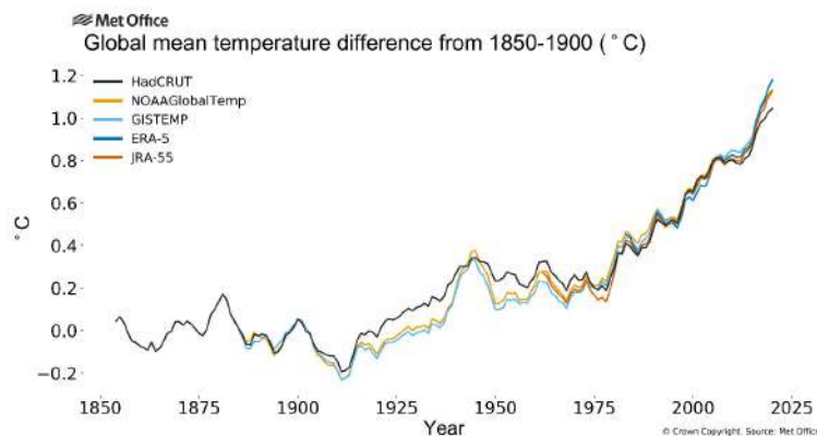
Figure 1: Five-year running average of global temperature anomalies (relative to pre-industrial) from 1854 to 2020 for five data sets: HadCRUT.4.6.0.0, NOAA GlobalTemp v5, GISTEMP v4, ERA-5, and JRA-55. Data for 2020 to June for HadCRUT4, and July for NOAA GlobalTemp, GISTEMP, ERA-5 and JRA-55.
