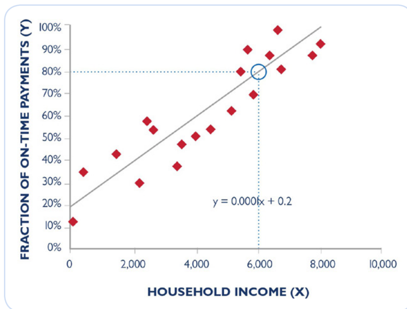
FIGURE 4: Illustration of a simple model that predicts on-time loan payments based on household income. In this very simple case, the model consists of a single equation, describing a linear relationship between income ( x ) and on-time loan payments ( y ). This model predicts that a household with an income of 6,000 will make 80% of their loan payments on time.
