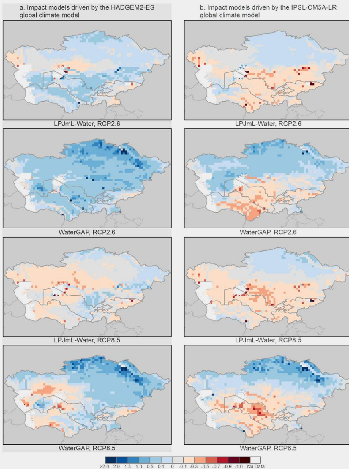
Figure A.9: ISIMIP average index values during 2010-2050 against 1970-2010 baseline for water availability, from LPJmL/water and WaterGap , forced with the HadGEM2-ES climate model (left) and IPSL-CM5A (right) under RCP2.6 and RCP8.5, Central Asia
