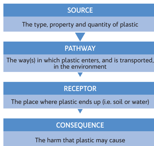
Figure 17: The source-pathway-receptor-consequence model
