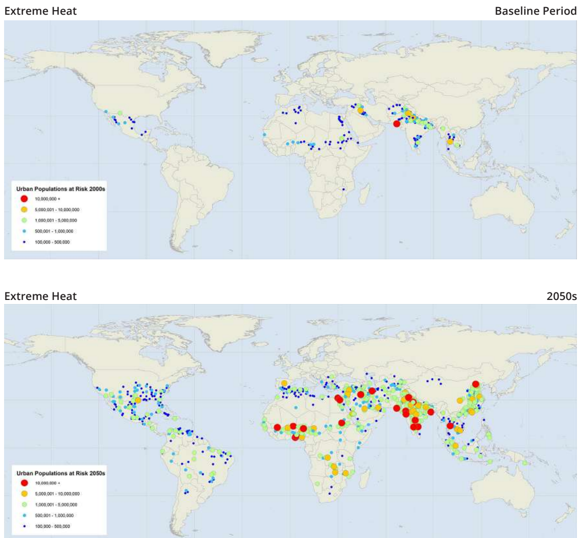
Figure 3. Urban populations at risk to extreme heat. Data source: Cities with a three month period (consecutive months) where average maximum temperatures exceed 35°C in the baseline period (top) compared to those that are projected to experience these temperature extremes by the 2050s (bottom). Multi-model mean temperature is derived from the NASA NEX-GDDP dataset with four GCMs (IPSL-CM5A-LR, MIROC-ESM-CHEM, GFDL-ESM2M, and NorESM1-M); Average monthly (hottest three consecutive months) maximum temperature for 1980-2005 baseline period is compared to 2041-2070 under RCP 8.5; Population estimates in the baseline period are from the Natural Earth Dataset for cities over 100,000 residents, and population growth rates for the 2050s are derived by applying the growth rate from the Global Rural-Urban Mapping Project (GRUMP) urban population extents to cities within the Natural Earth Dataset.
