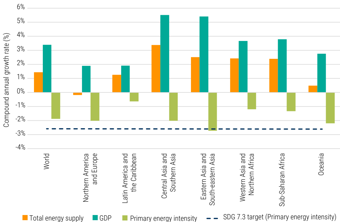
Figure 4.4 • Growth rate of total energy supply, GDP and primary energy intensity at a regional level, 2010-19
