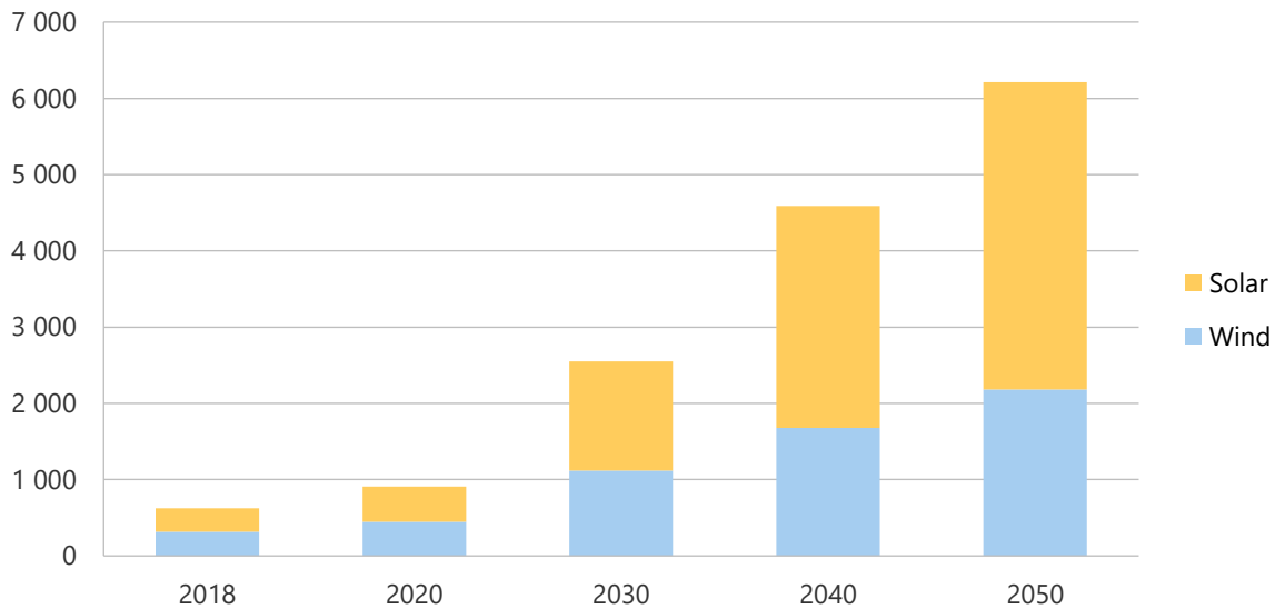
Figure 7-6. Wind and solar PV generation capacity in CN, 2018-2050 (GW).
