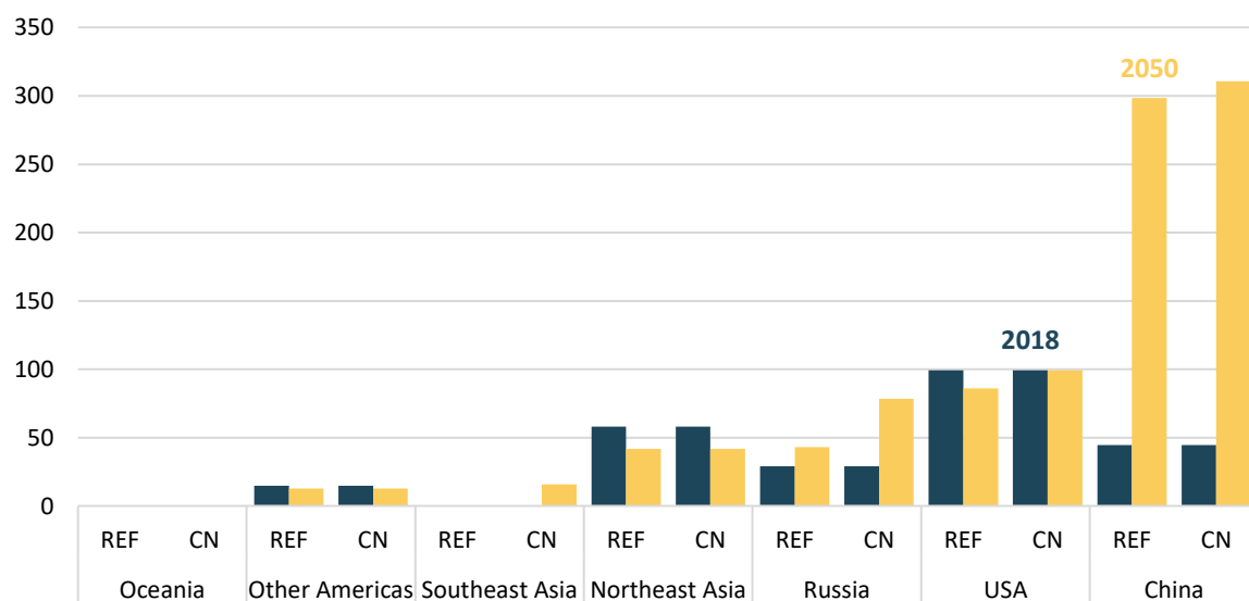
Figure 6-12. Installed nuclear capacity in REF and CN, 2018 and 2050 (GW).
