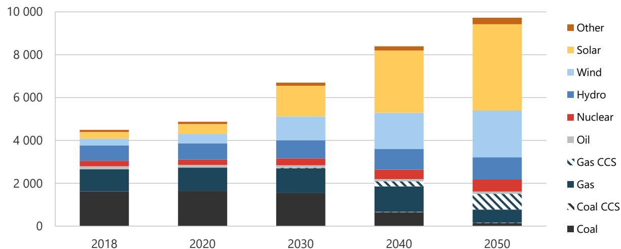
Figure 3-6. Generation capacity in CN, 2018-2050 (GW).
