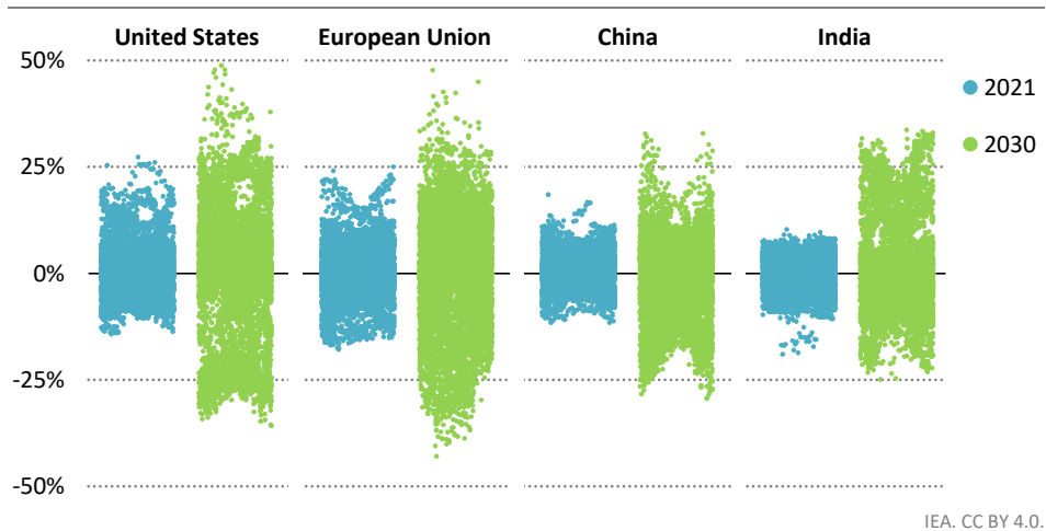
Figure 6.16 ▶ Hour-to-hour flexibility needs in the United States, European Union, China and India in the APS, 2021 and 2030
