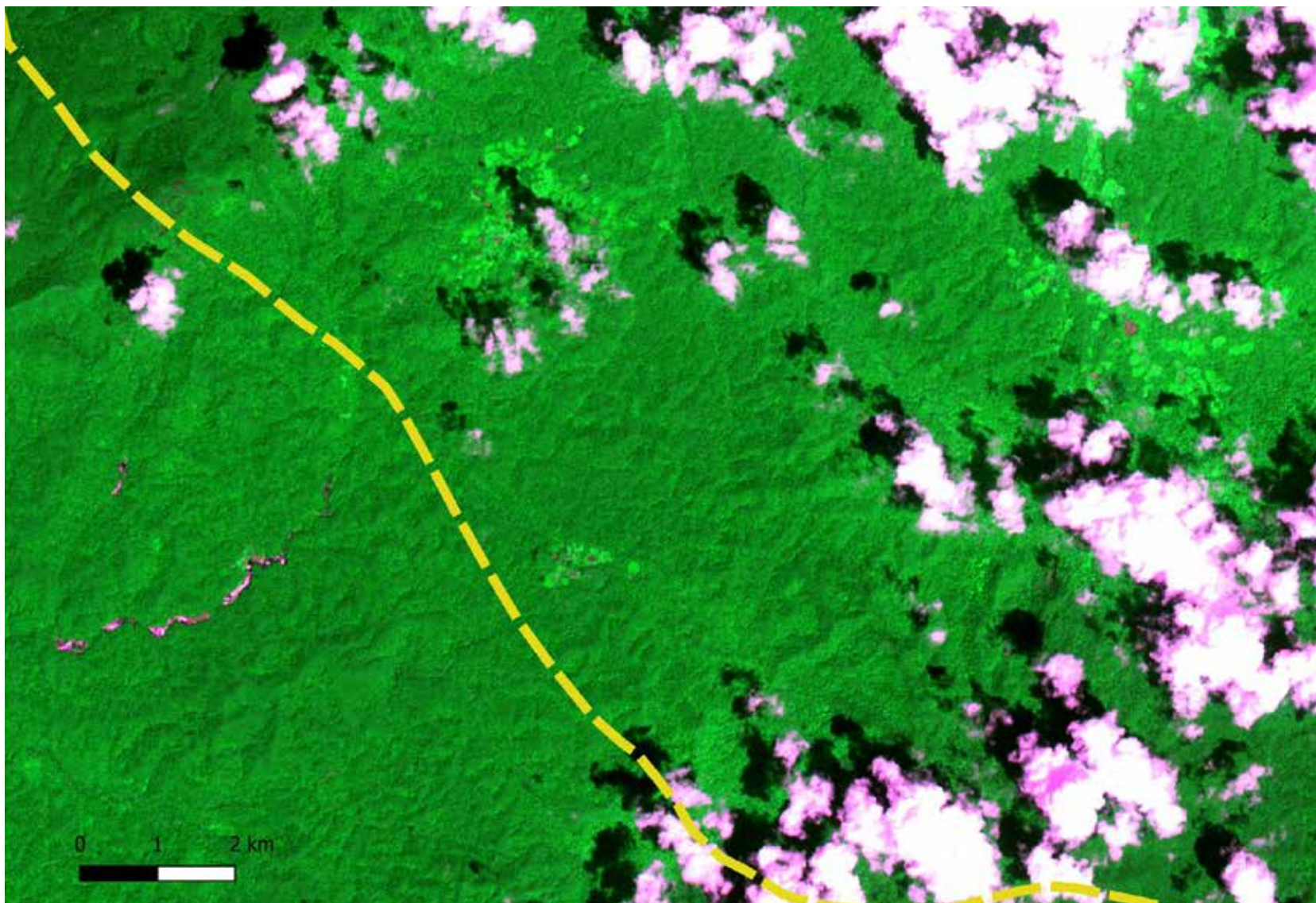
Image 3: Sentinel 2 satellite mosaic from November 2021.
