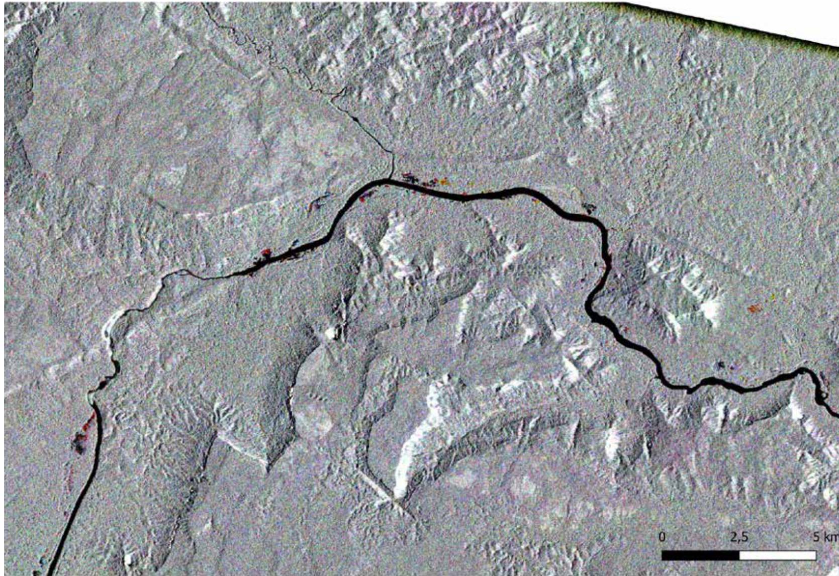
Image 2: Multitemporal mosaic of radar images in 2021 of the confluence of the Aracaça and Uraricoera rivers.
