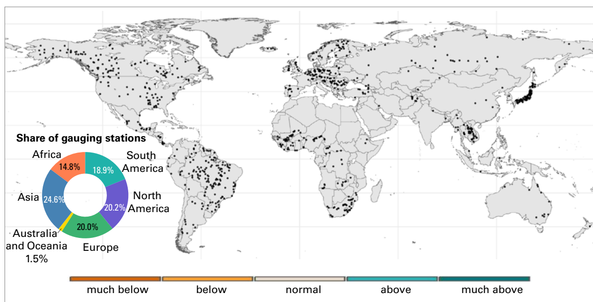
Figure A3. Location of gauges for which data were obtained from the Remote Sensing-based Extension of GRDC (RSEG)
