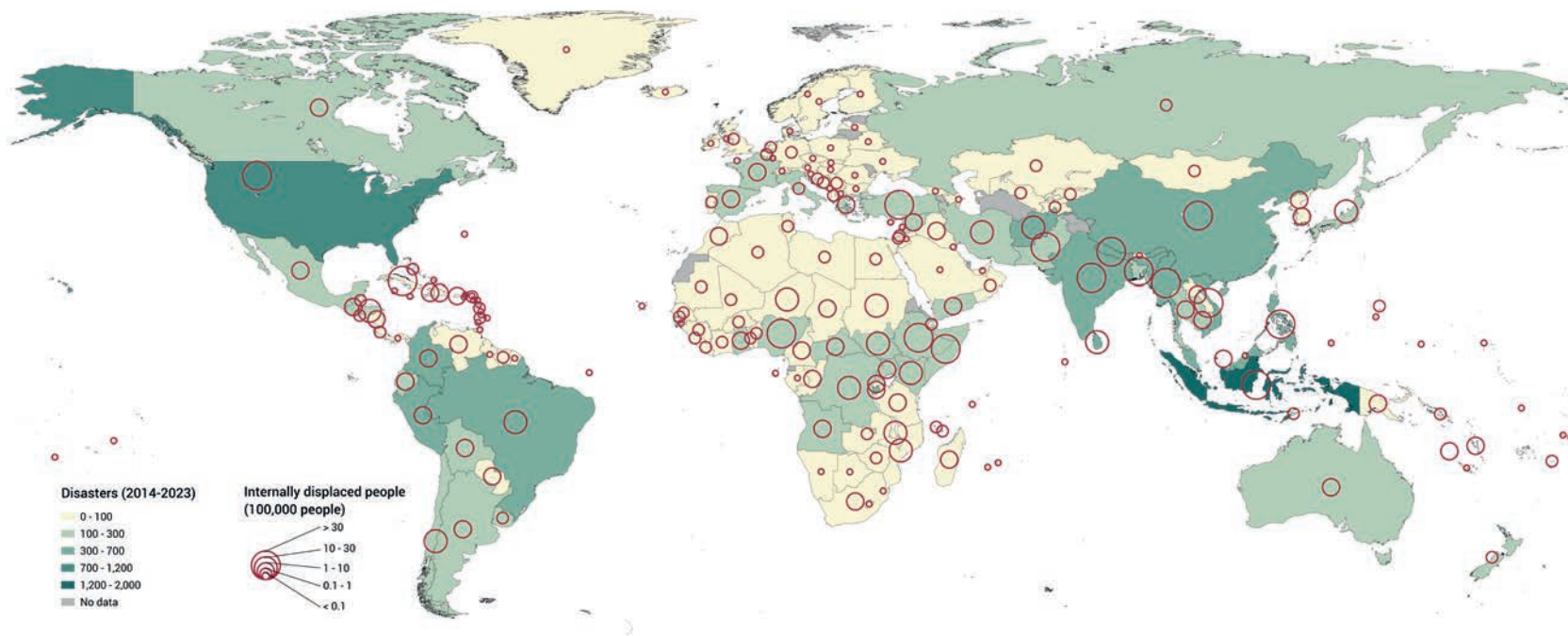
Map 2. Number of forced movements of internally displaced people by disasters 2014–2023
