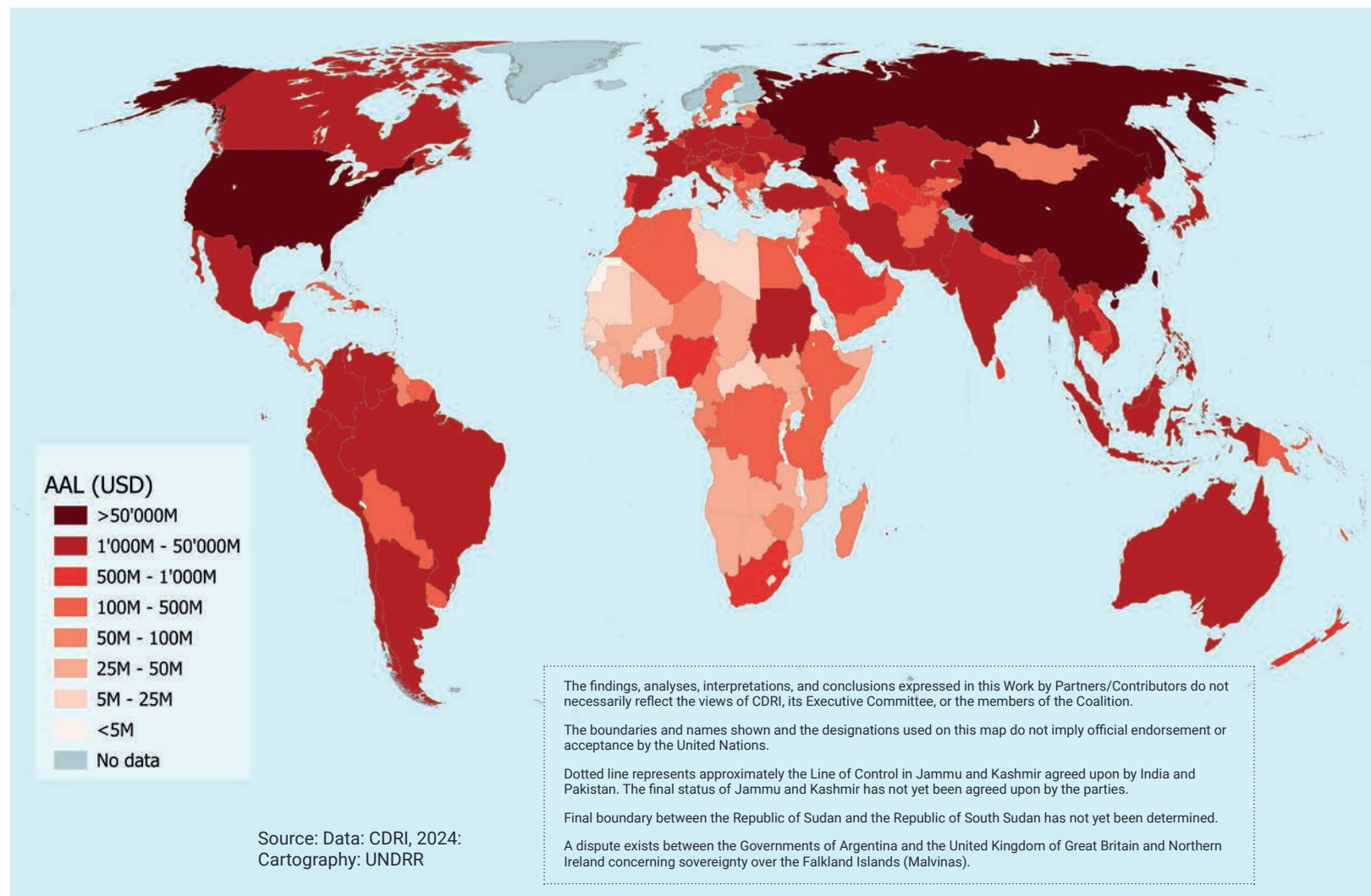
Map 26. AAL by floods and cyclones within the critical infrastructure sectors
