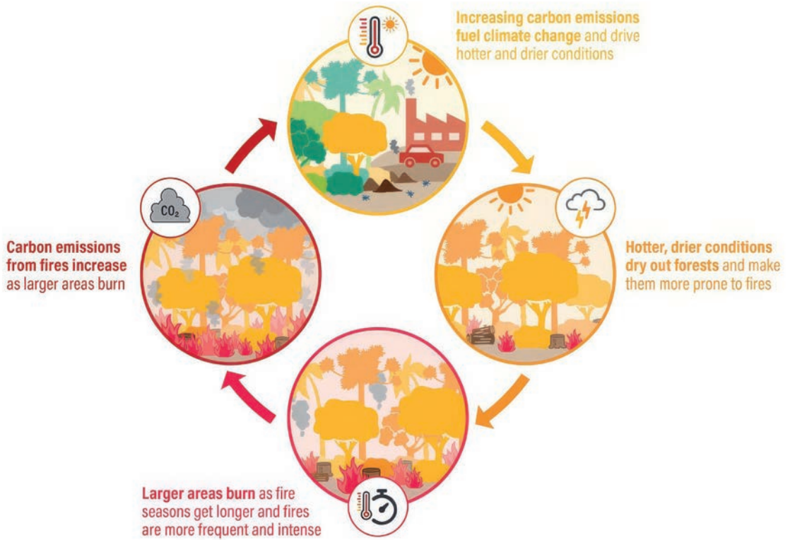
Figure 25. Fires and the climate feedback loop
