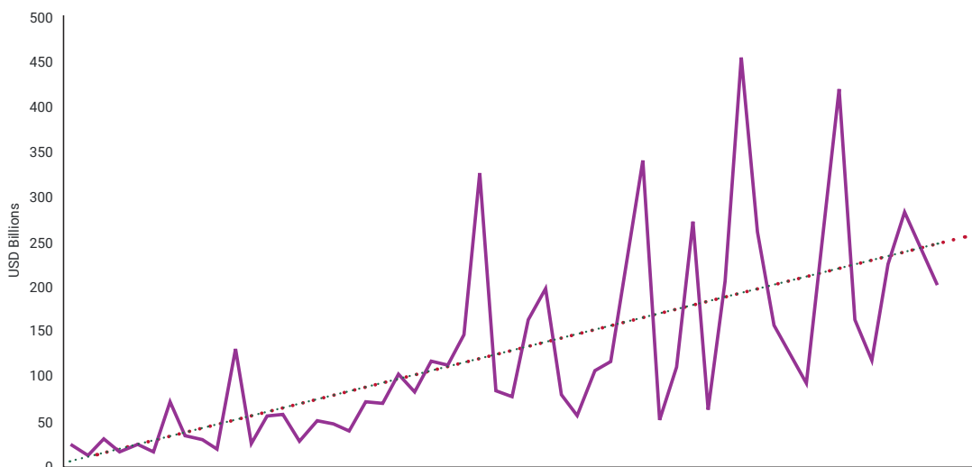
Figure 2. Rising direct costs of recorded disasters 1970 – 2023
