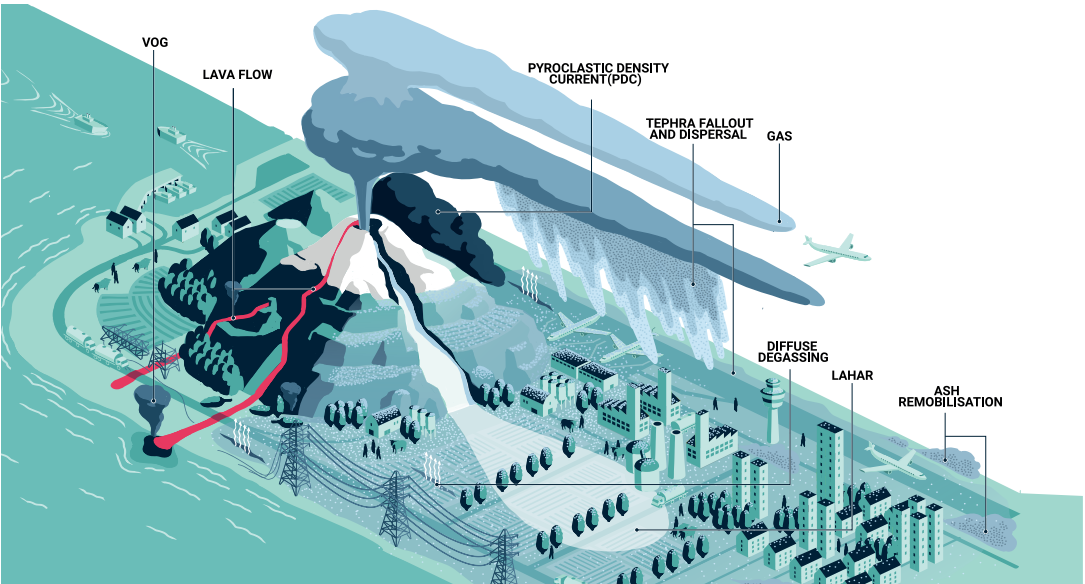
Figure 19. Volcanic risk and its potential impacts
