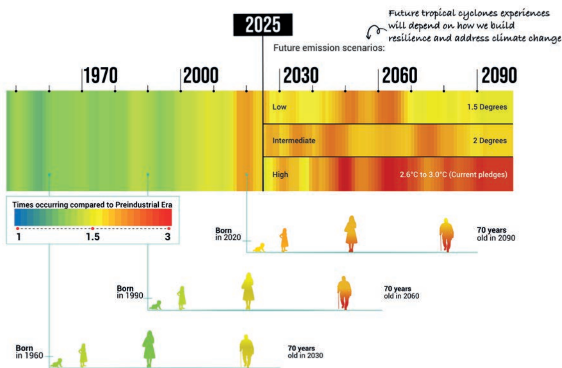
Figure 42. Projected lifetime probability of experiencing a 1-in-100-year tropical cyclone event
