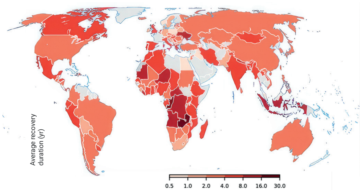
Map 22. Average post-disaster recovery duration, by country & Figure 23: Median recovery duration by country income group
