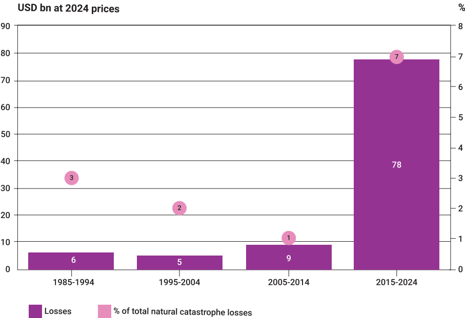
Figure 36. Global insured losses from wildfires
