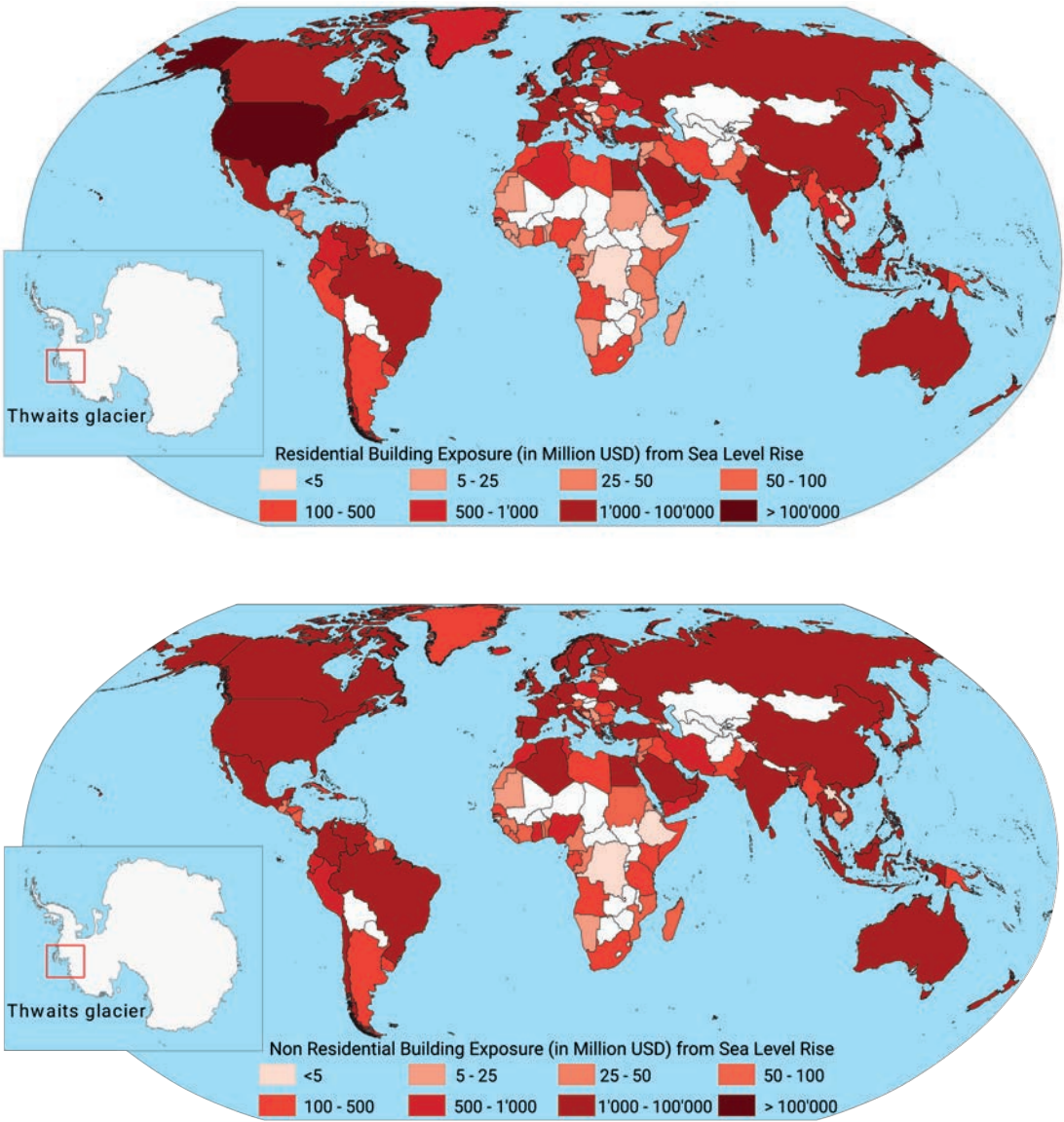
Map 5. Modeled economic losses to residential and non-residential buildings associated with a potential collapse of the Thwaits Glacier
