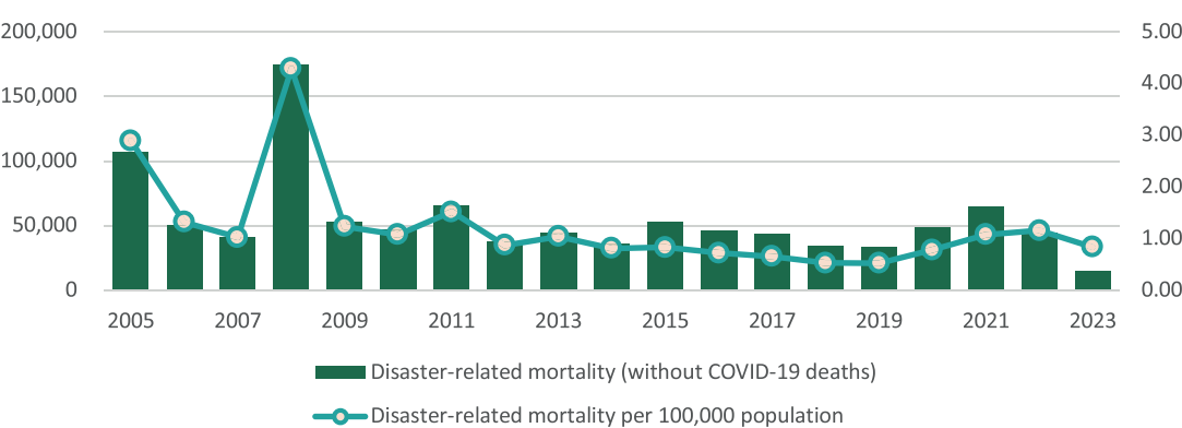
Figure 1. Disaster-related mortality worldwide, 2005–2023
