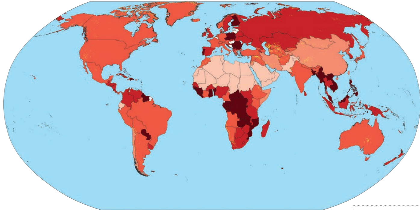
Map 42. Global desertification rates, 2003–2022
